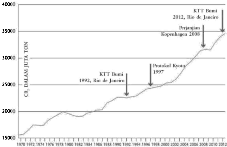
EMISI CO 2 GLOBAL, 1970–2013
